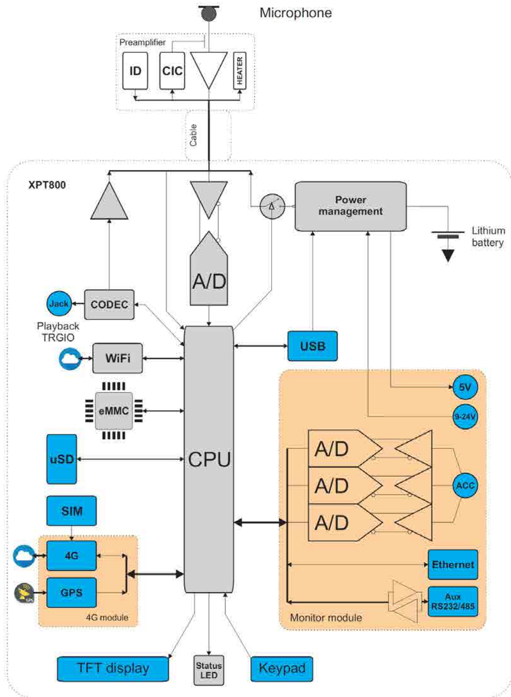
Fig. 2 - Block diagram
